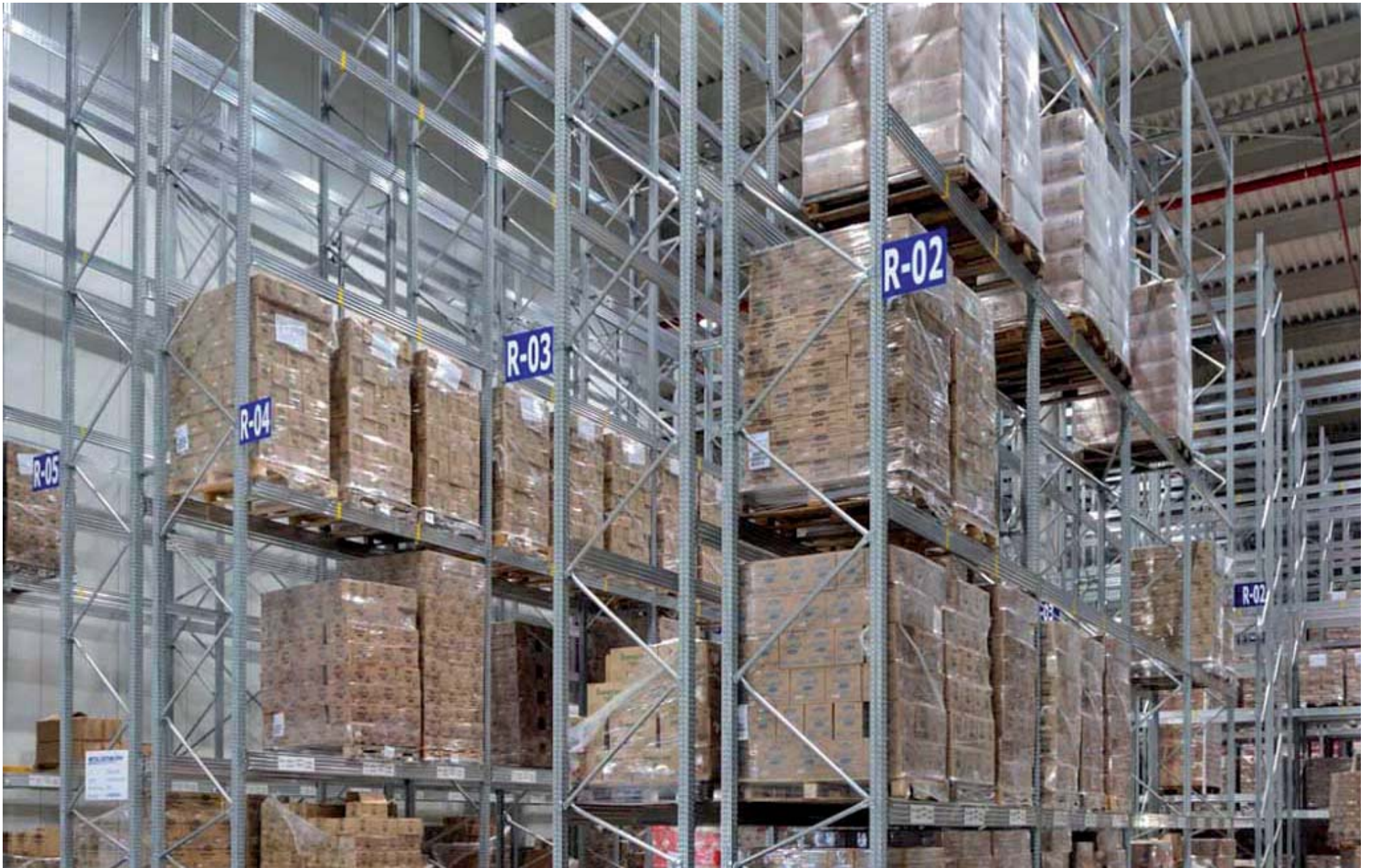
3-PL-Warehouse equipped with roller conveyors and METALSISTEM's "SUPER 4-5-6" Pallet Racking Series <October 2012>
